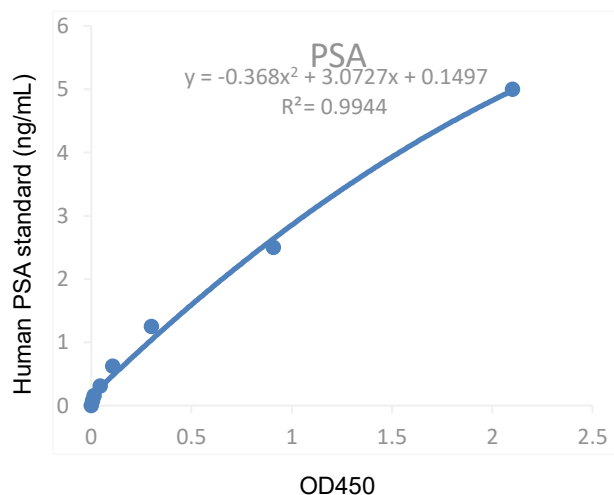
Figure. Standard Curve of Human Prostate Specific Antigen (PSA) in 96-well plate assay, data provided for demonstration
